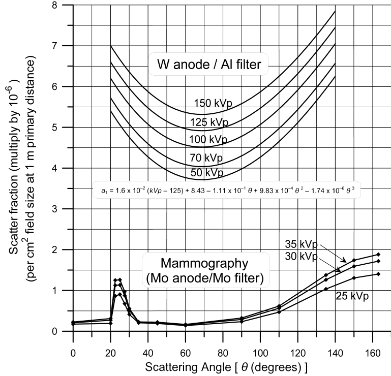
Fig. C.1. The scatter fraction a_1 \times 10^{-6} (i.e., multiply graph value by 10^{-6} ) per \text{cm}^2 of primary beam area at 1 m. [Data of Trout and Kelley (1972) reanalyzed by Simpkin and Dixon (1998) for tungsten anode, aluminum-filtered beams. Data of Simpkin (1996b) for molybdenum anode, molybdenum filtered mammographic beams.]
