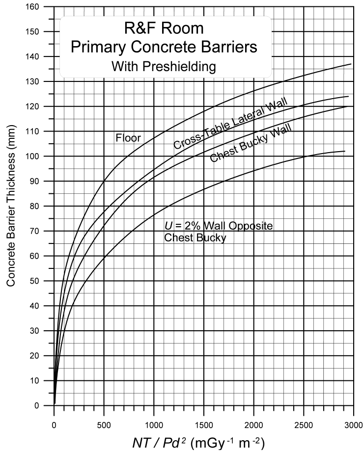
Fig. 4.8b. The concrete (standard-weight) thickness requirements for primary barriers assuming preshielding ( x_{\text{pre}} ) in the representative R&F room shown as a function of NT/Pd^2 (see Section 4.1.6.2 for caveats on x_{\text{pre}} ). P is in milligray per week, N is the weekly total number of patients examined in the R&F room, and d (in meters) is chosen as the distance from the most intense radiation source to the occupied area. Image-receptor data as in Figure 4.5b. If the W_{\text{norm}} values given in Table 4.5 do not match the per patient workload for the facility under consideration, then the original value of NT/Pd^2 can be multiplied by W_{\text{site}}/W_{\text{norm}} , and the modified value can be used to obtain the required shielding from Figure 4.8b.
